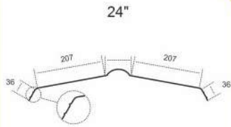
Roll Formed Ridge (Option 1)
